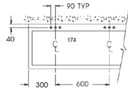
Typical tap hole dimensions and centres
