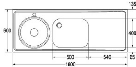
Left Hand Sluice Top Entry
